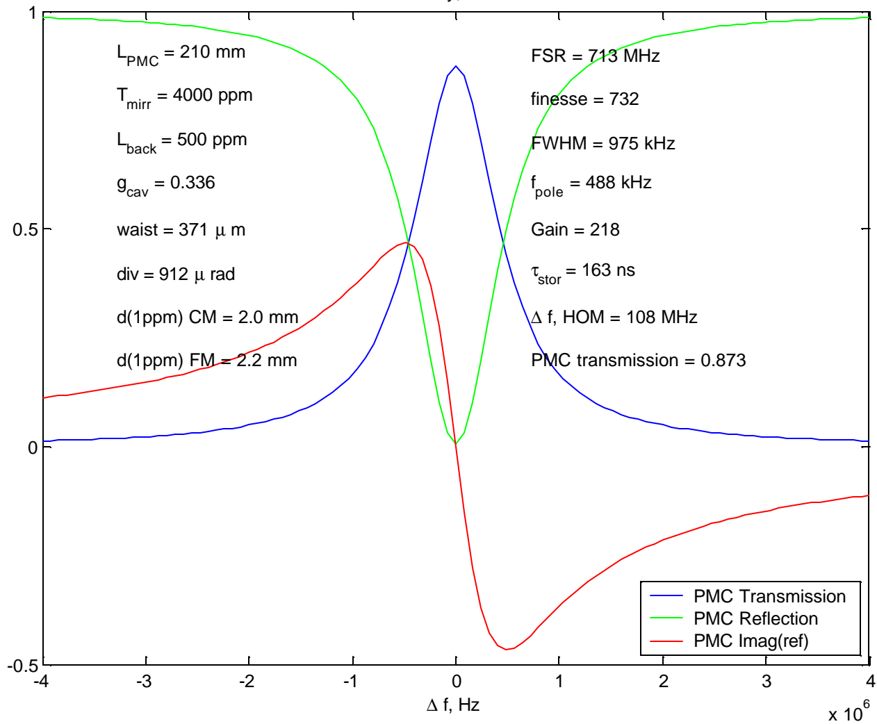
PSL PMC cavity, as built at 40m
